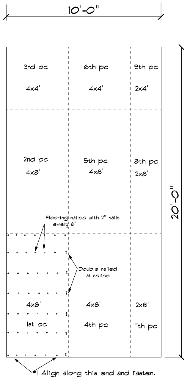
10x20' Sample Floor Layout
