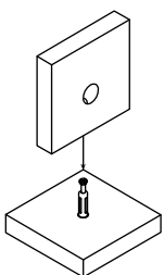
4. Installation plate
