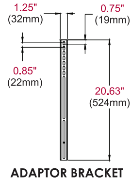
ADAPTOR BRACKET
