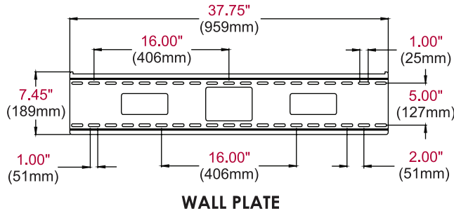
WALL PLATE
