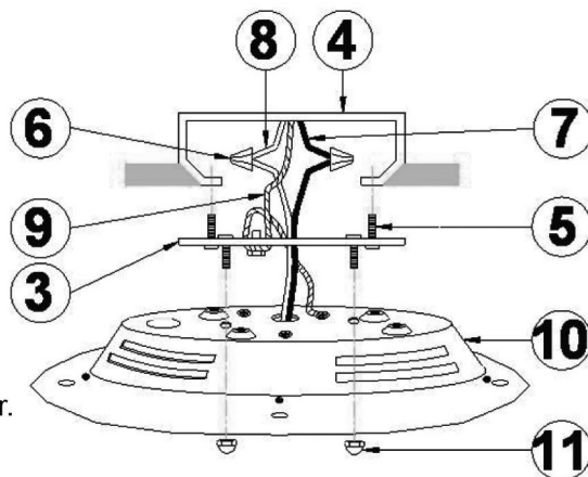
Ceiling Outlet Box
