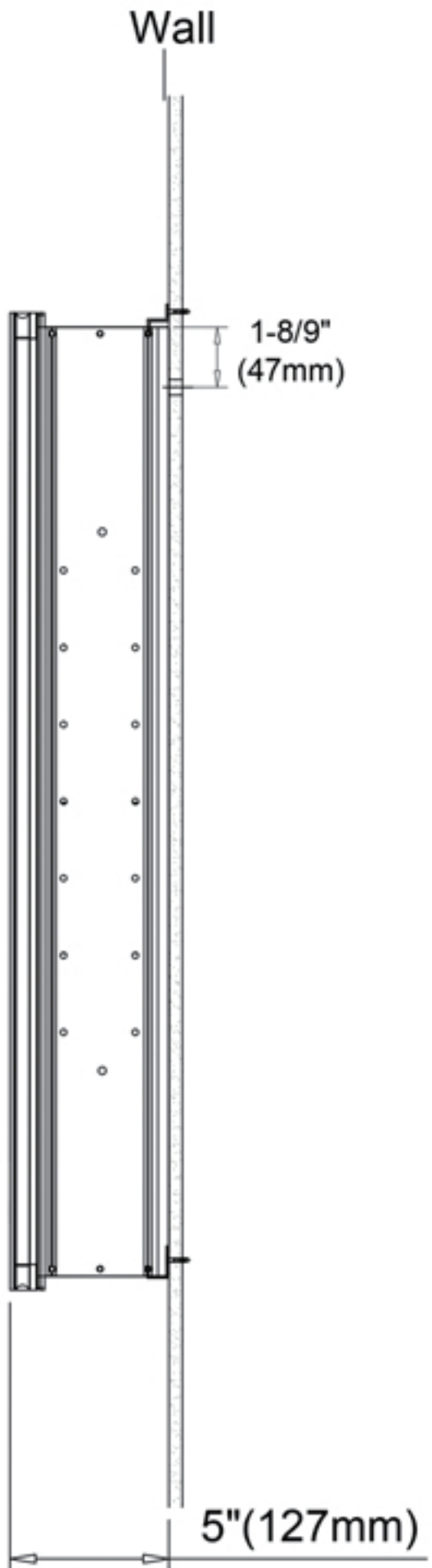
Surface Mount
