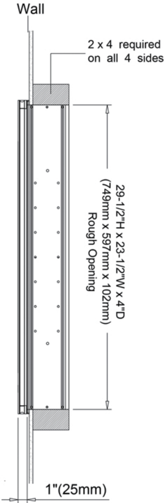
Recessed Mount
