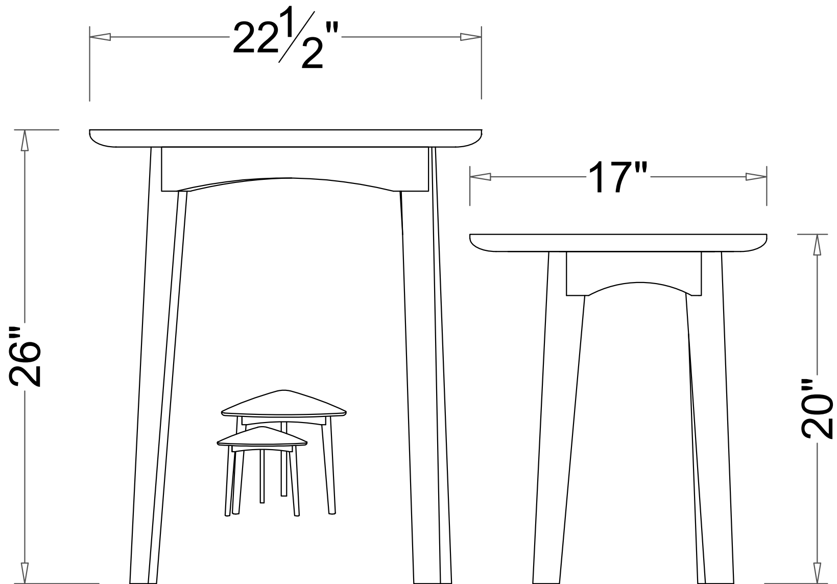
Nesting Table
