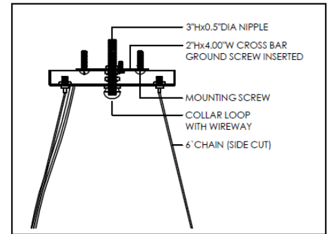
CANOPY DETAILS
