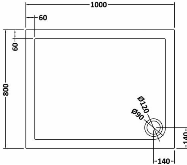
1000 x 800 RECTANGULAR TRAY
