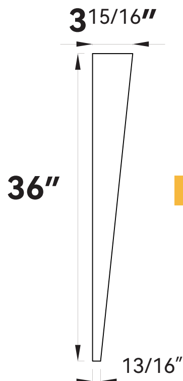
SIDE VIEW
