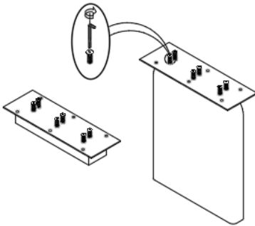
1x1024 Hexagon screw Øx30
