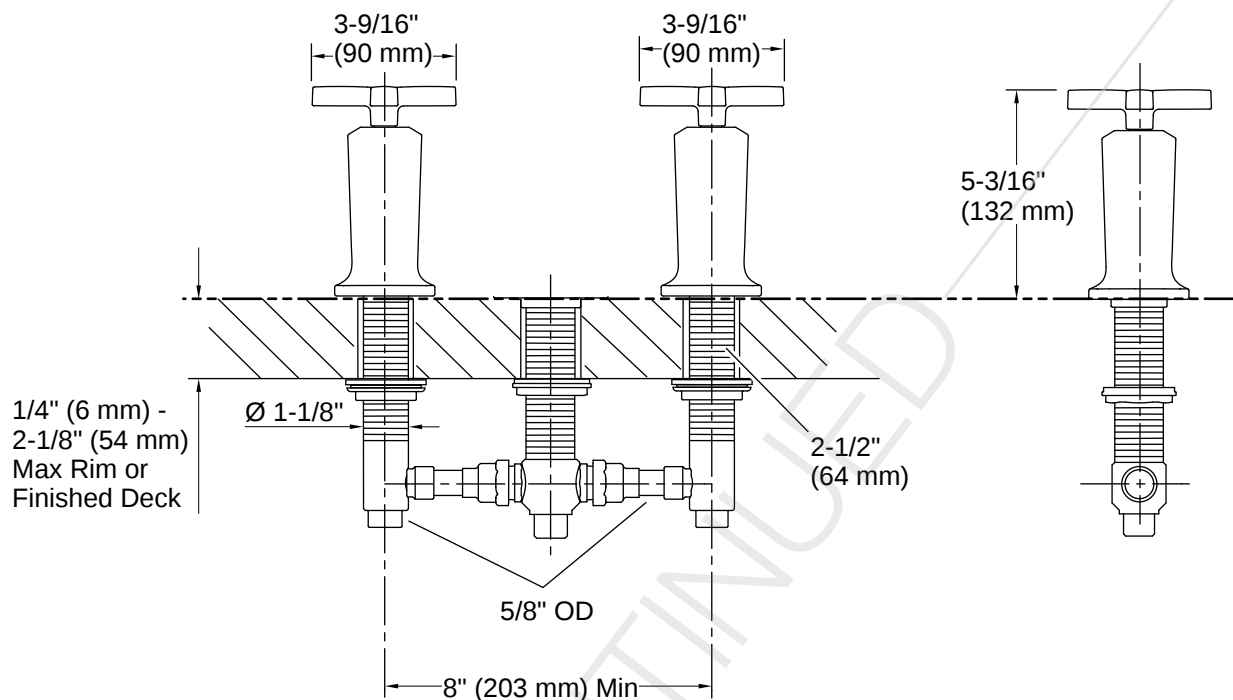
Rim or Finished Deck Mount Installation
