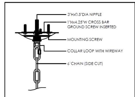
CANOPY DETAILS
