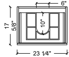
TOP VIEW WITHOUT COUNTER
