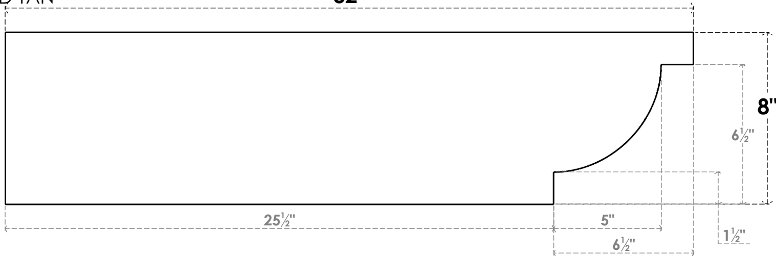
SIDE PROFILE
