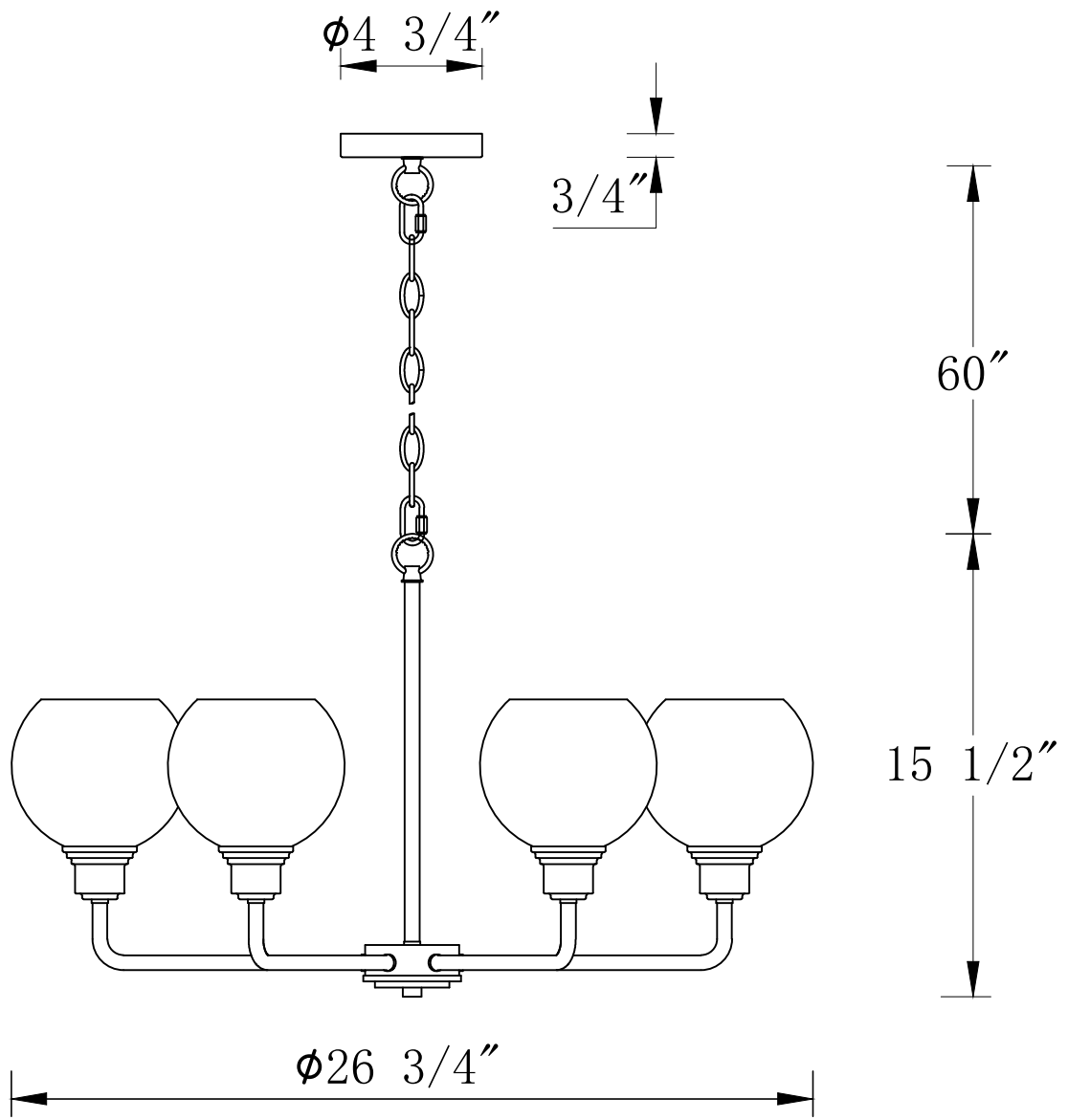
FRONT VIEW
