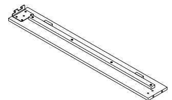
O. SIDE RAIL 1 2 pcs
