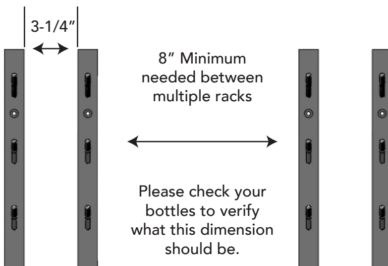
Diagram A: Mounting Dimensions
