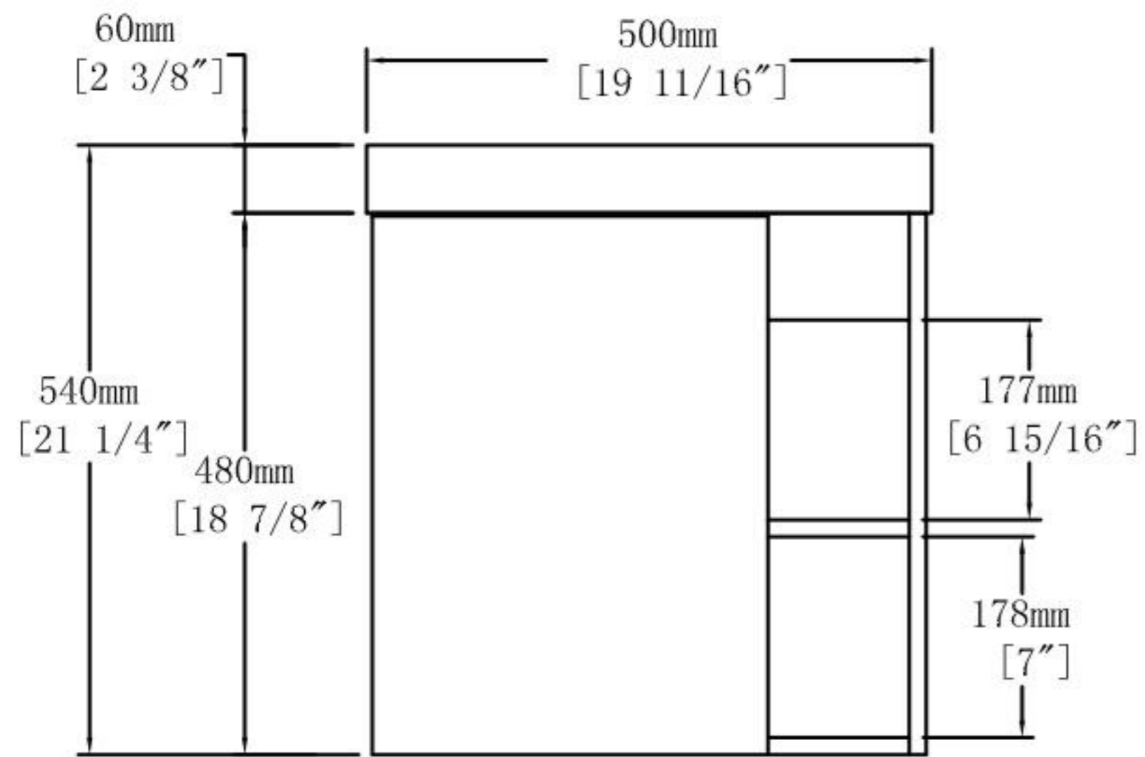
Front View
