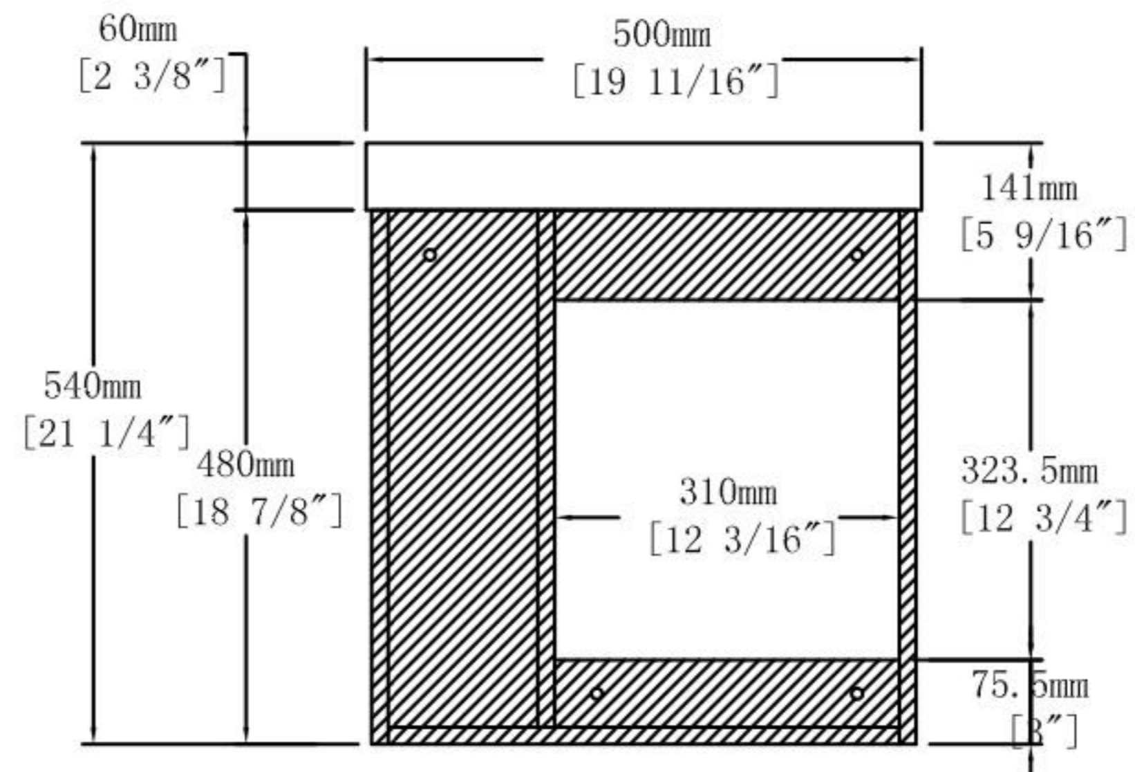
Back View
