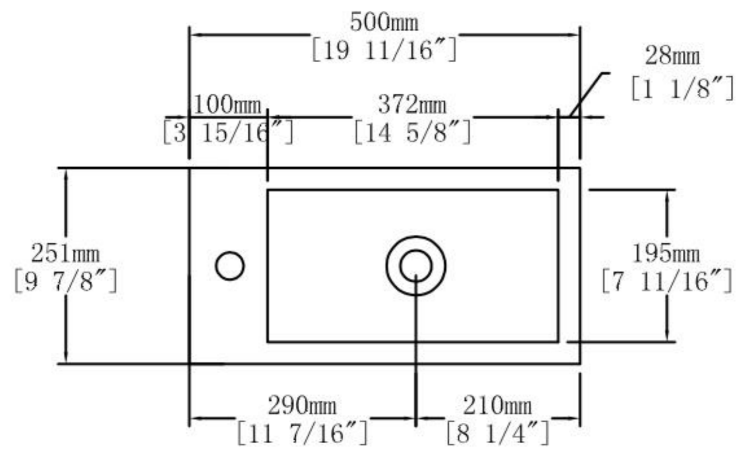
Top View
