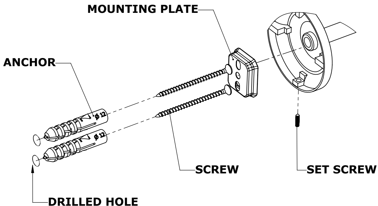
DETAIL M
