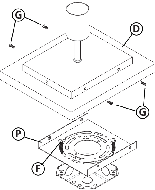
JUNCTION BOX
