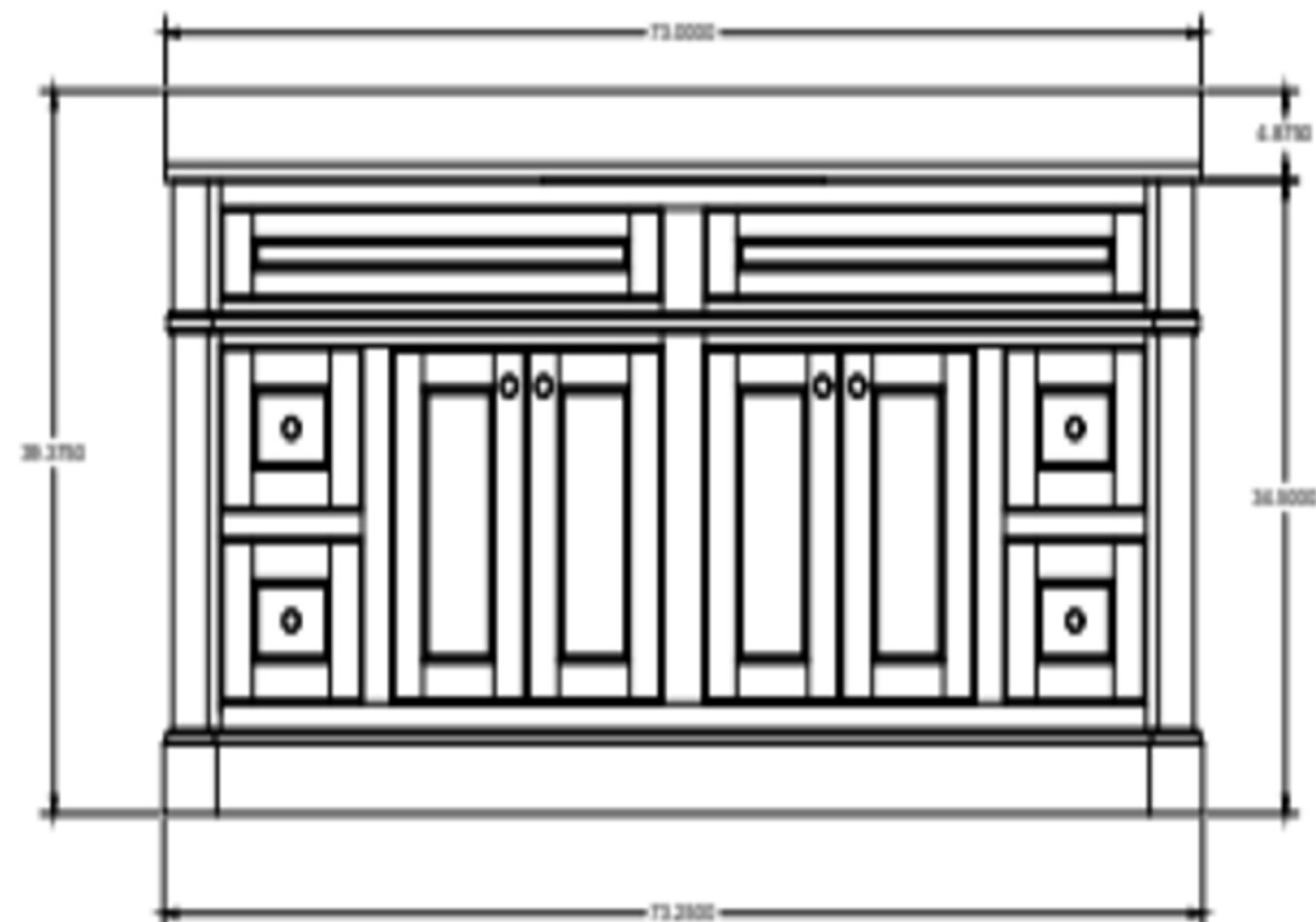
FRONT VIEW
