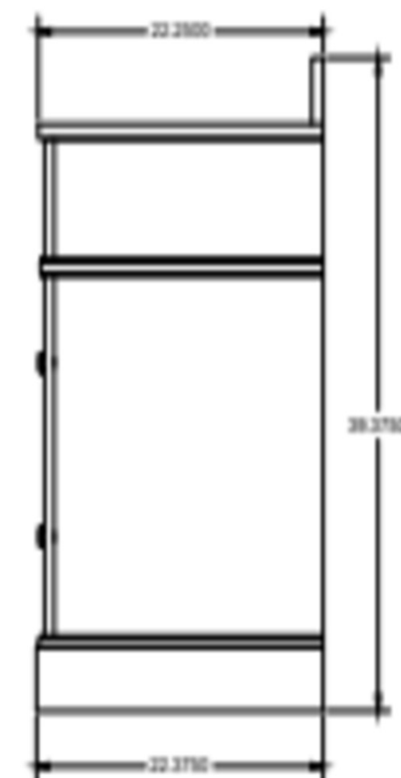
SIDE VIEW
