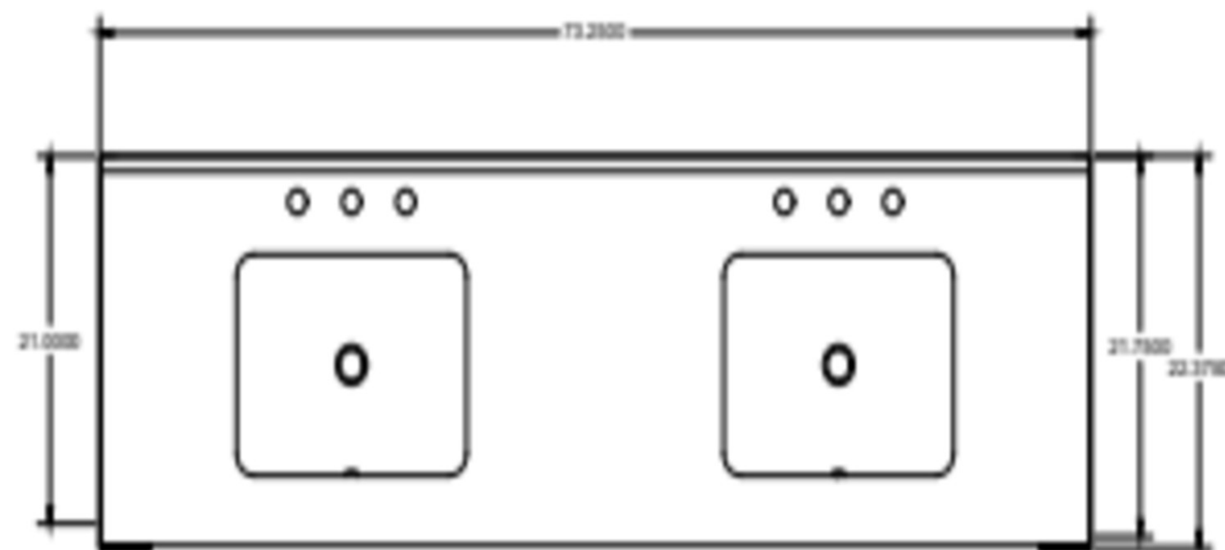
TOP VIEW
