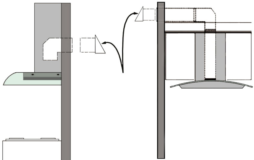
TOP VENTING WALL EXHAUST
