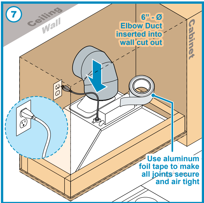
(7) Connect the range hood to a designated standard outlet. Check the fan motor and lights are functioning. Use aluminum foil tape to make all joints secure and air tight.
