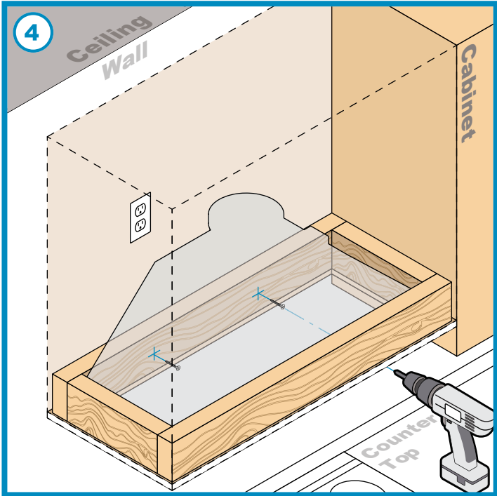
(4) Through the installation holes, fasten the range hood using #8 2-1/2" (minimum) woodscrews to mount onto the wood blocking.
