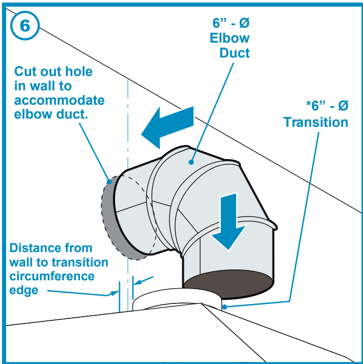
(6) Minimum distance from wall to transition circumference edge will be 2 3/4". This will depend on how much space is provided with wood blocking and range hood placement.
