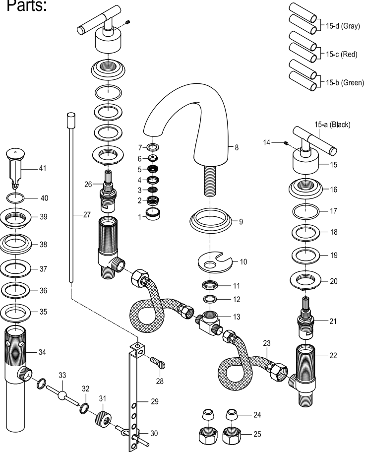
Hot Cartridge: KSRPL5000HC
