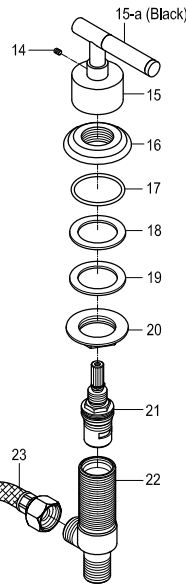
Cold Cartridge: KSRPL5000CC
