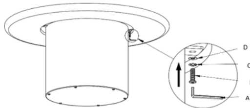
Insert the bolts through washers onto the top. But be careful not to overly tighten them as concrete might crack
