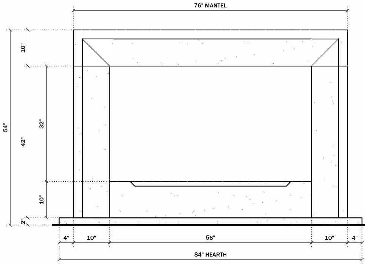
FRONT ELEVATION
