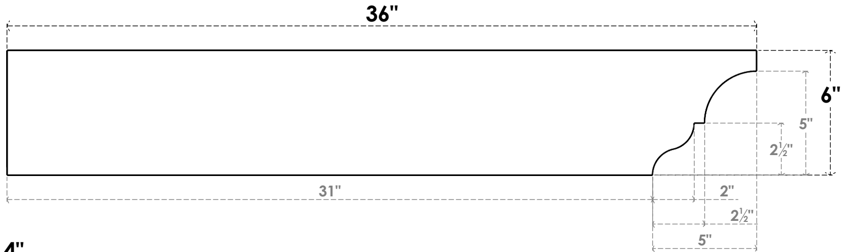
SIDE PROFILE
