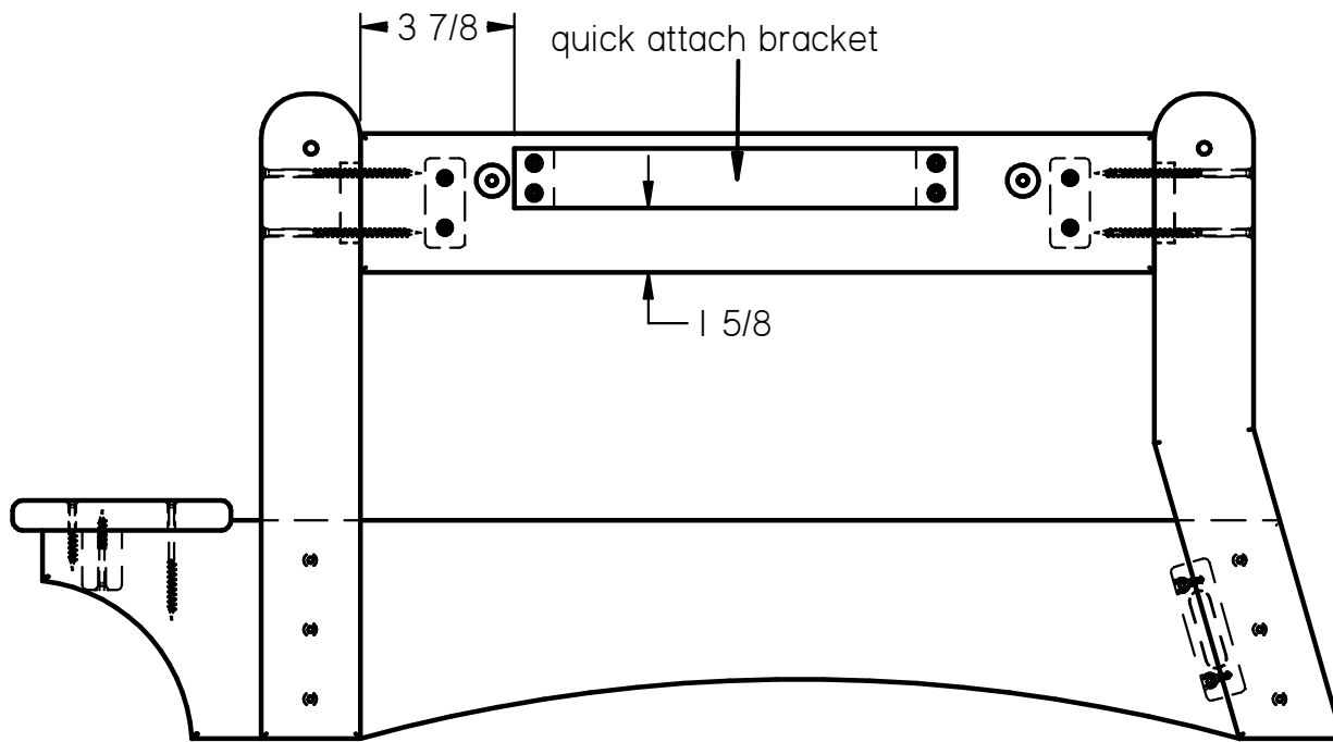
Template to attach Gliding Settee Table brackets to Counter Height Gliders
