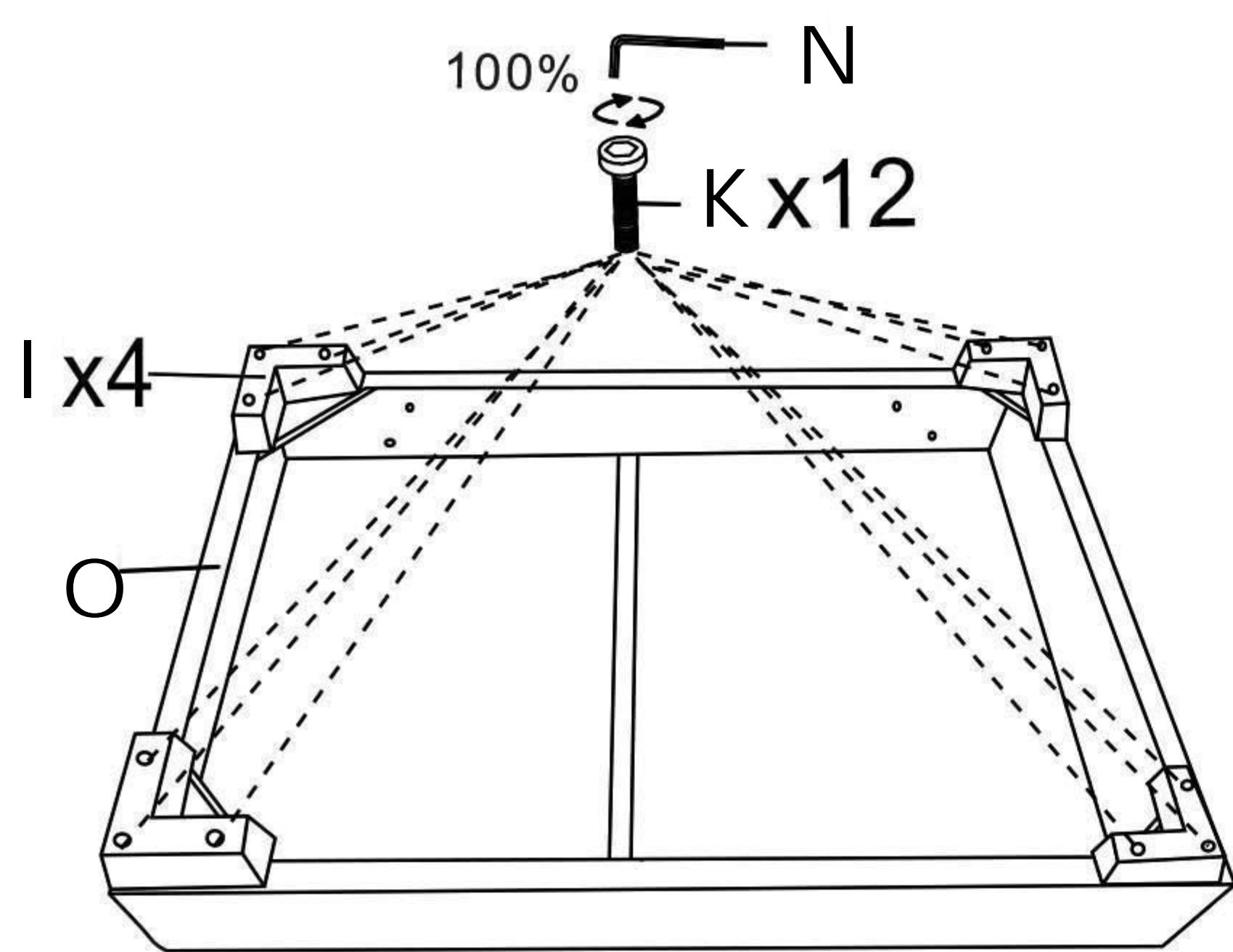
Seat frame 1
