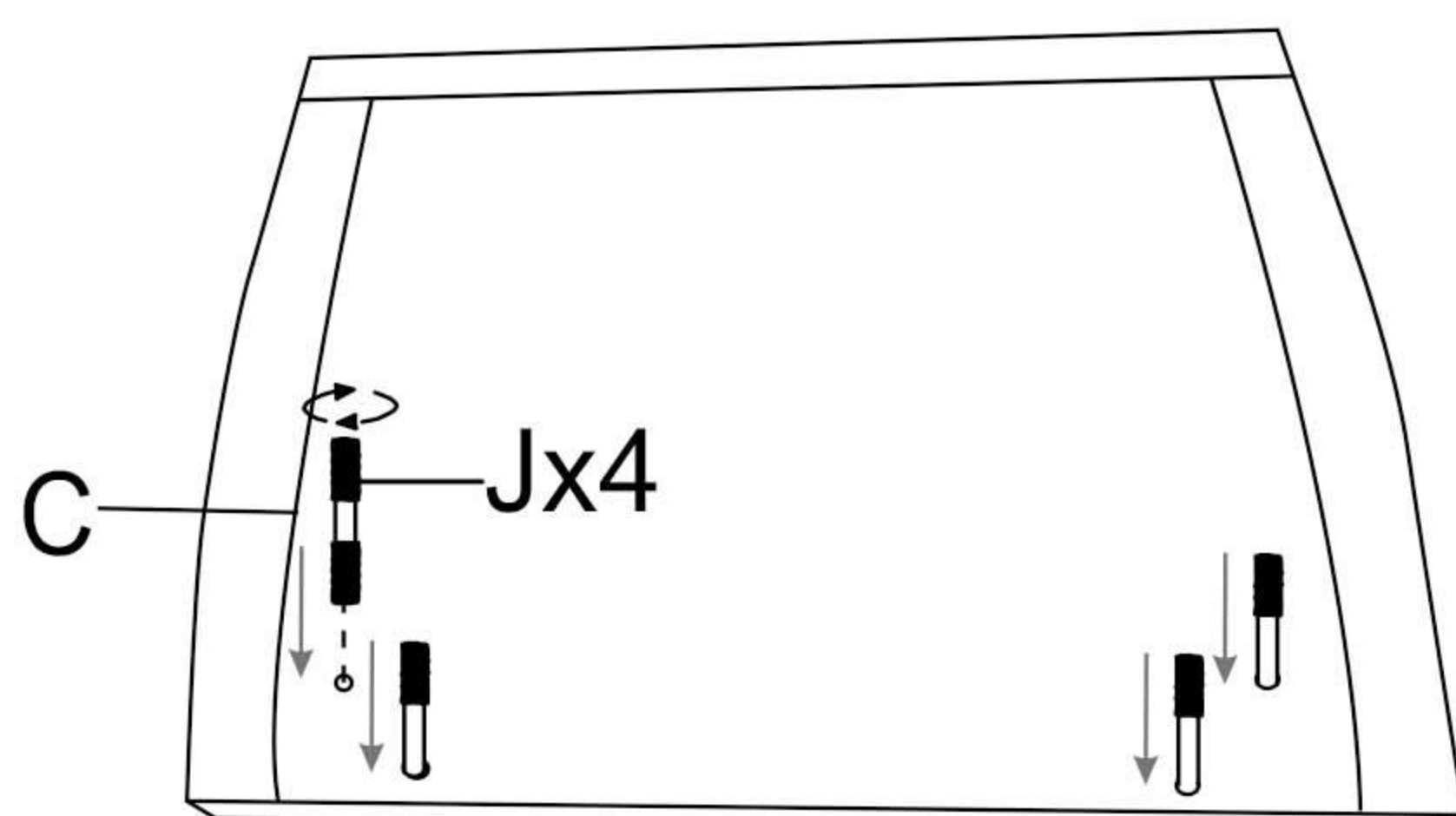
Backrest 1
