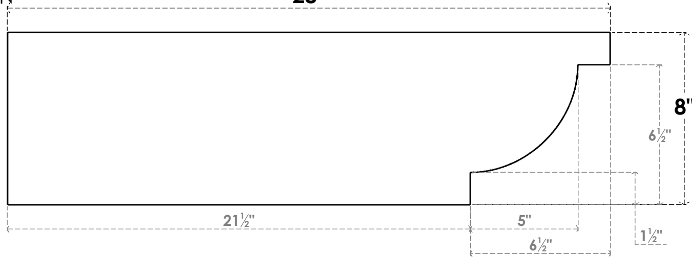
SIDE PROFILE
