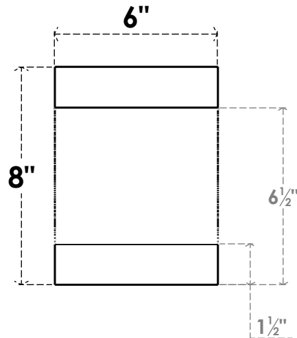
FRONT PROFILE
