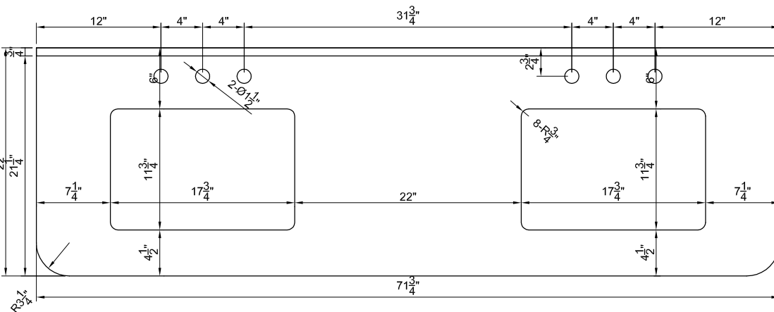
TOP VIEW OF VANITY CABINET
