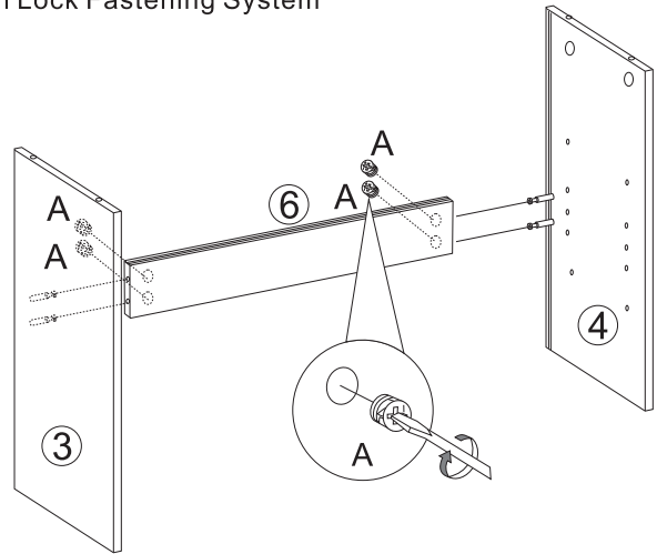
Cam Lock Fastening System
