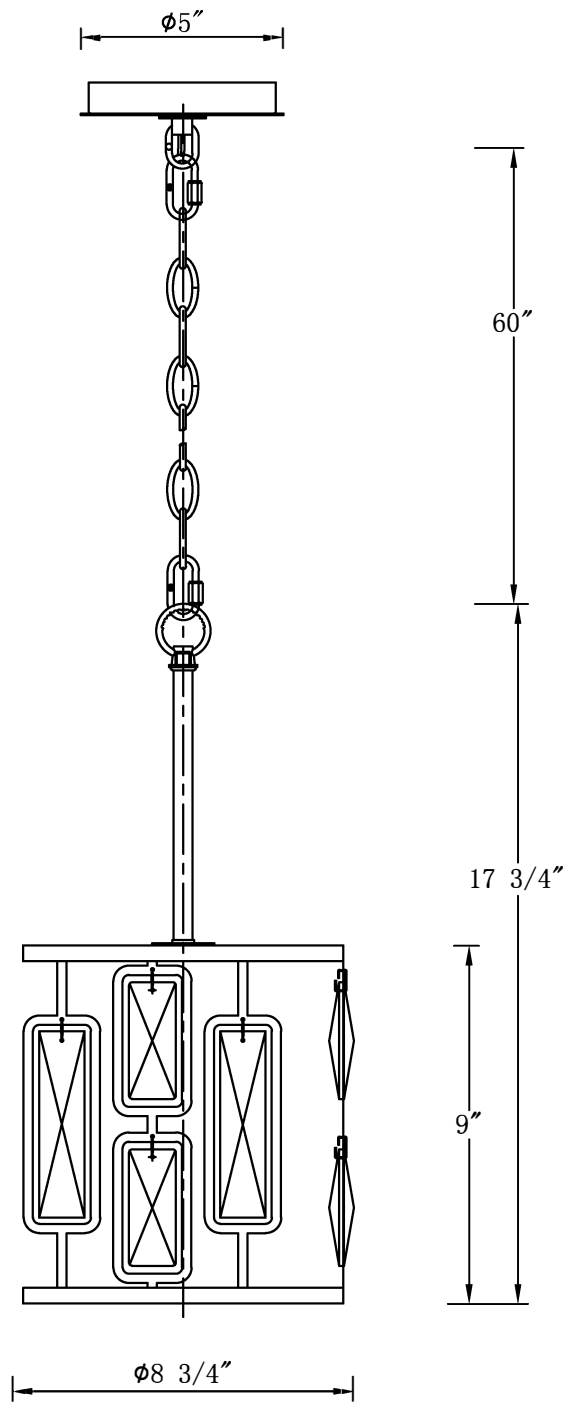
FRONT VIEW
