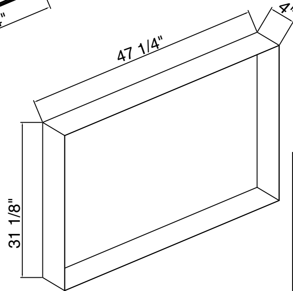
759048-LED-MC
