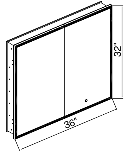
759036-LED-MC
