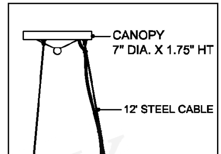
CANOPY DETAIL
