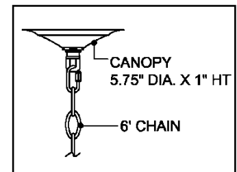
CANOPY DETAIL
