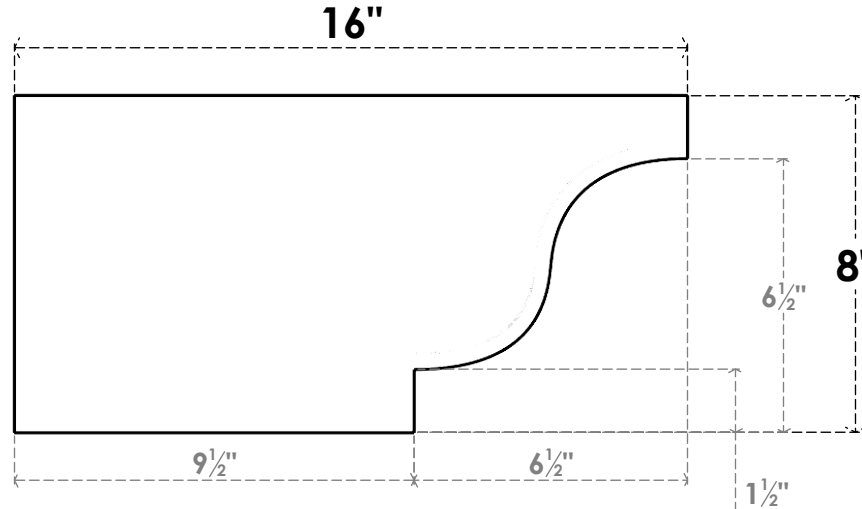
SIDE PROFILE
