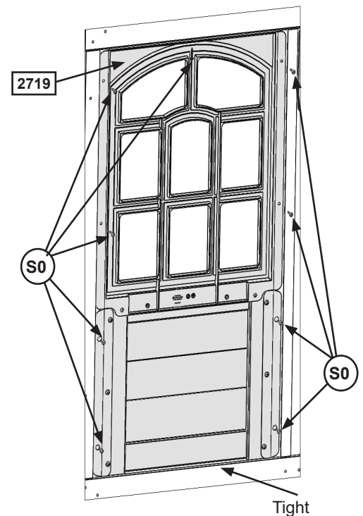
Fig. 11.7 Inside View
