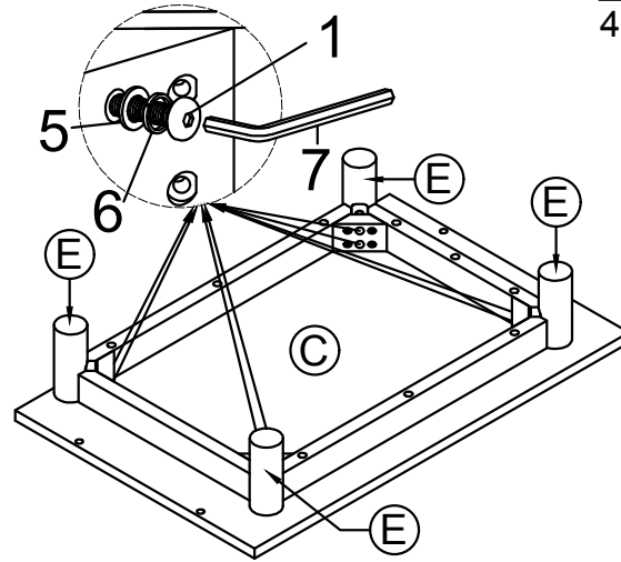
STEP 1: 8 Point - Bolt 1/4"x50mm
