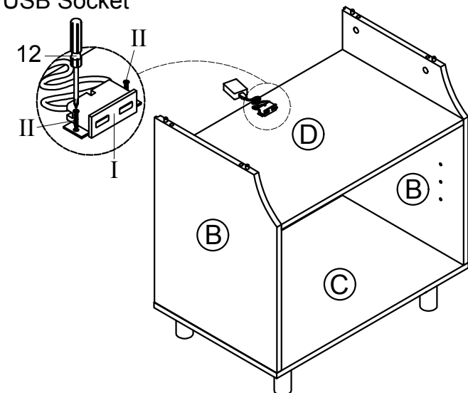
STEP 5: Assembly USB Socket
