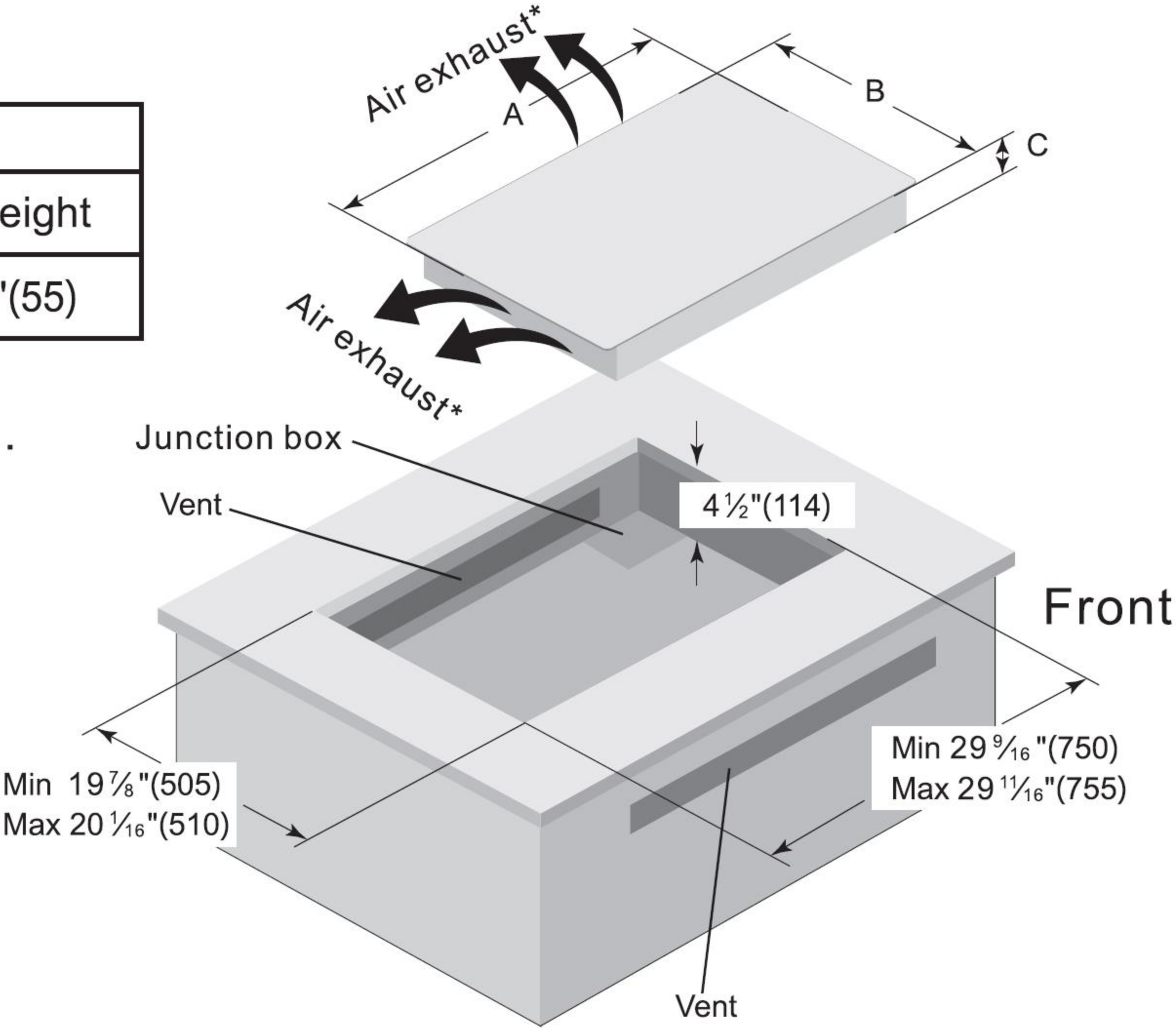
EMPV-IDC30 Cooktop and Cutout Dimension
