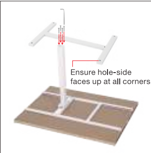
STEP 8 Use 4 long screws to connect hinge and H-base frame. Ensure all screws are fully tightened.
