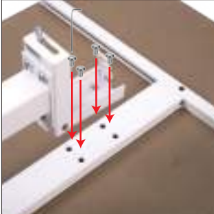
STEP 4 Use 4 short screws to connect Tabletop and hinge as shown
