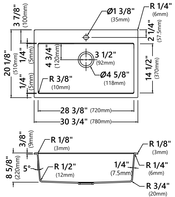
Model #: KGD-412B Sink Dimensions: 33" x 22" x 9 3/4" Min Cabinet Size: 36"
