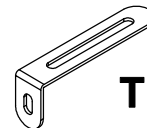
S x 2
