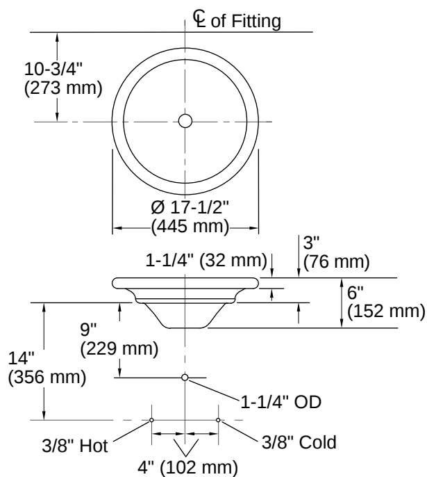
Standard Installation
