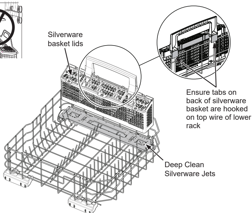
Silverware Basket - 10 Place Settings Models - GD*650, GD*665, GD*670, PD*715
