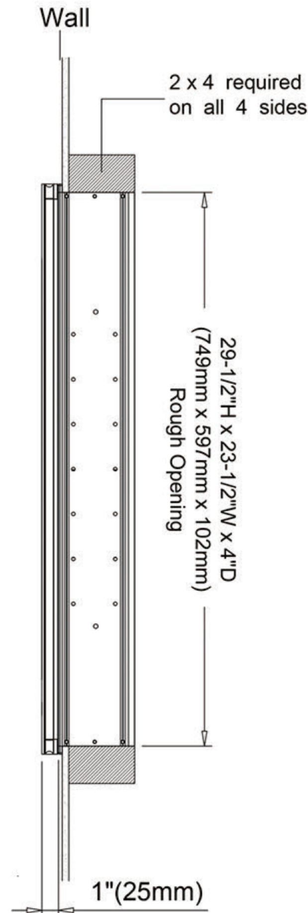
Recessed Mount
