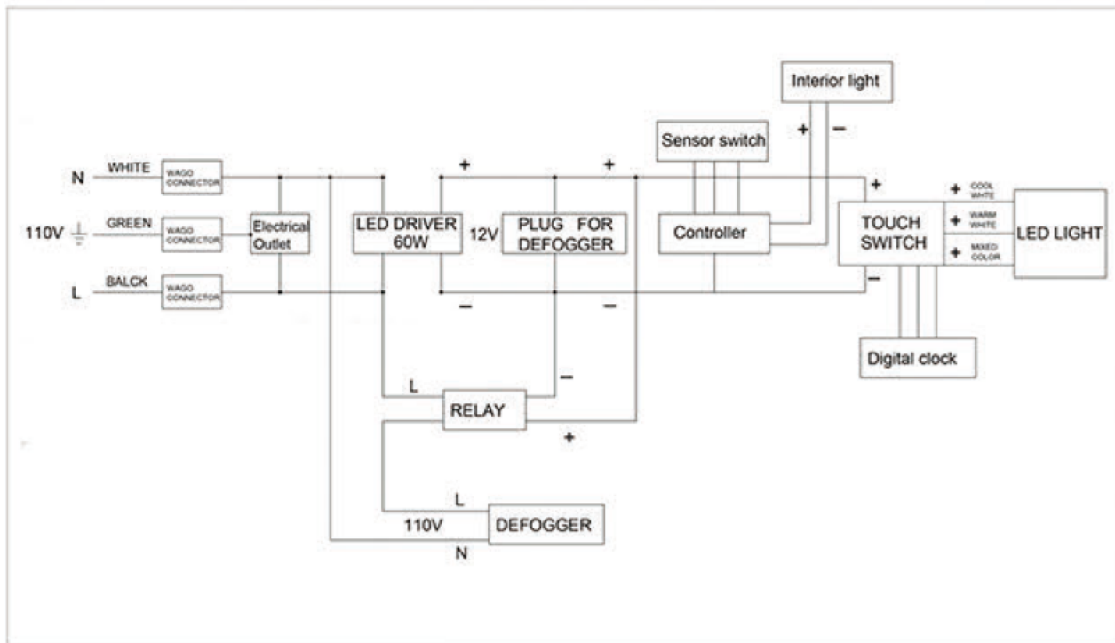
Circuit Diagram
