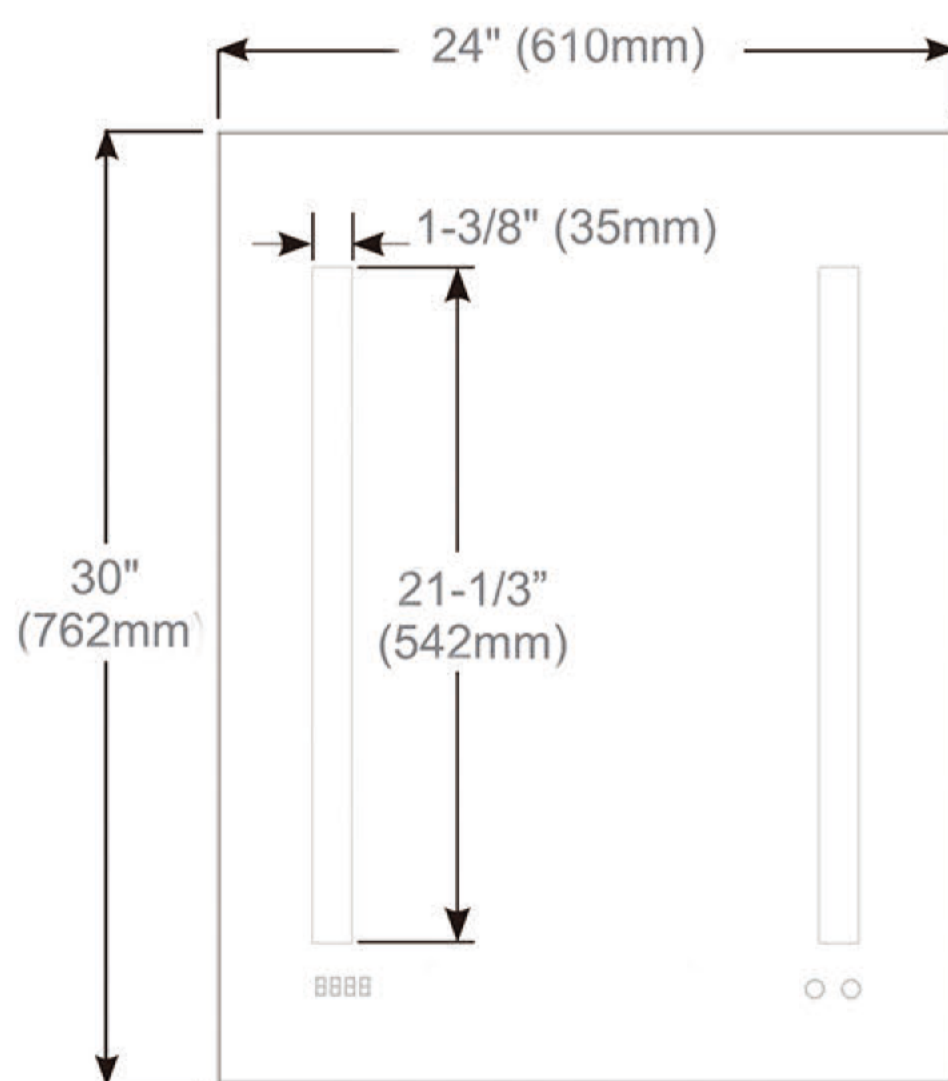
Cabinet Dimensions
