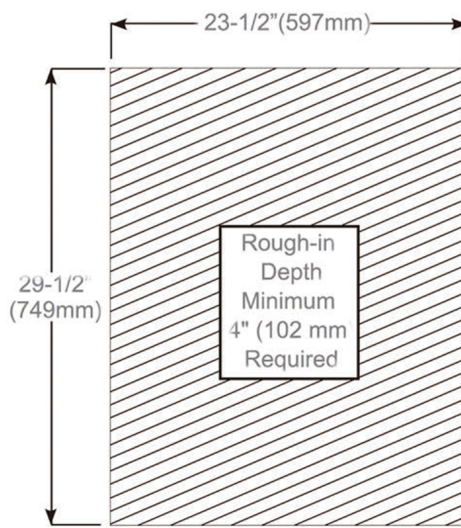
Rough-in Dimensions
