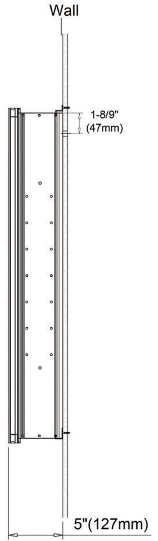
Surface Mount
