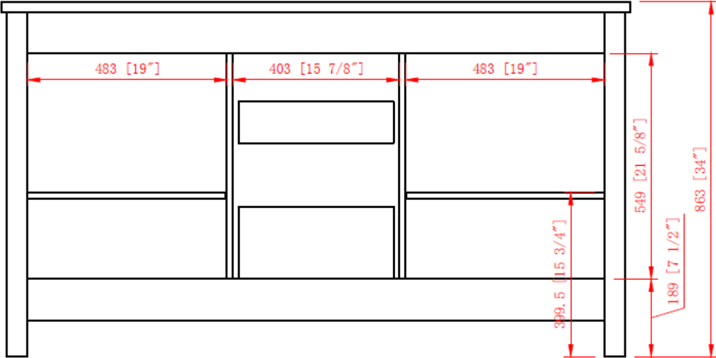
BACK VIEW
