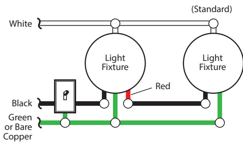
Wiring Diagram 1
