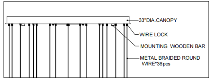
CANOPY DETAIL
