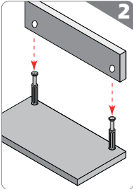
Cam screw
